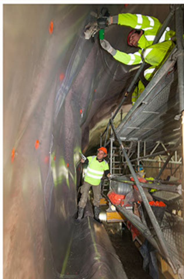
Tunnel du Siaix (étanchéité SOPREMA) © Laurent FABRY - Studio ARLY PHOTOGRAPHY http://bit.ly/2UQk7Su
